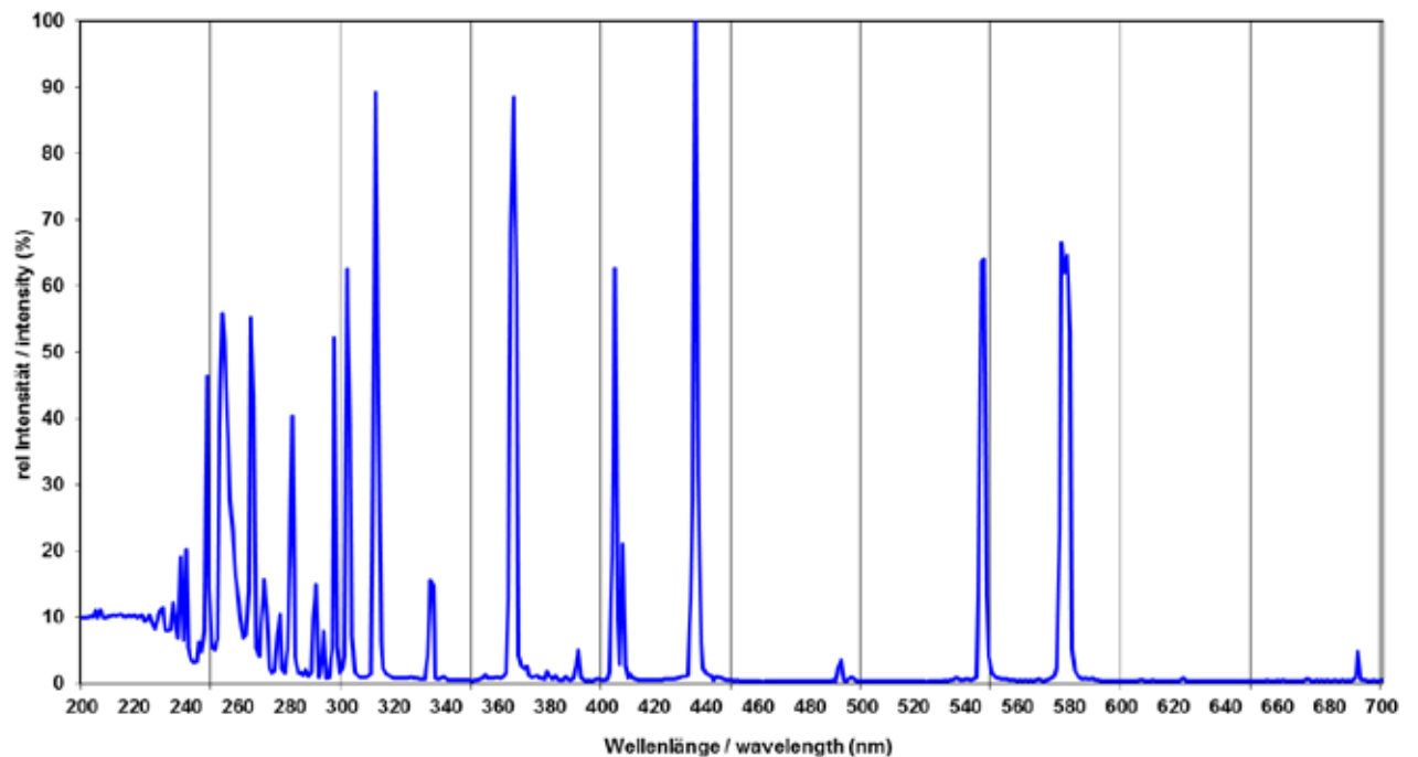
Spektrum Standard Hg (mercury) 100 W/cm
