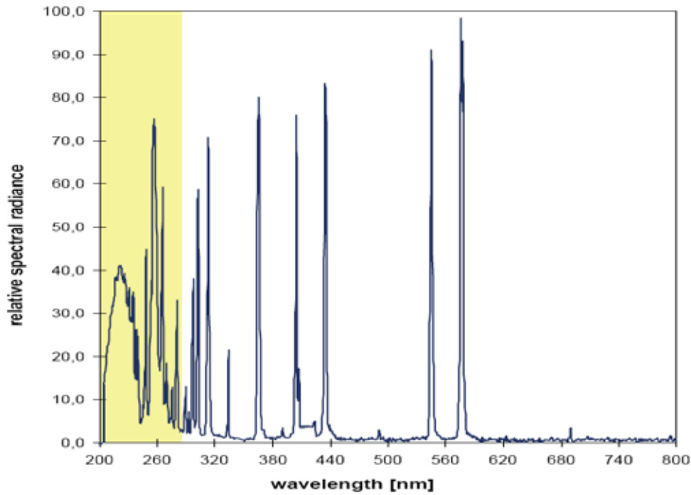
Spektrum Standard Hg (mercury) 100 W/cm
