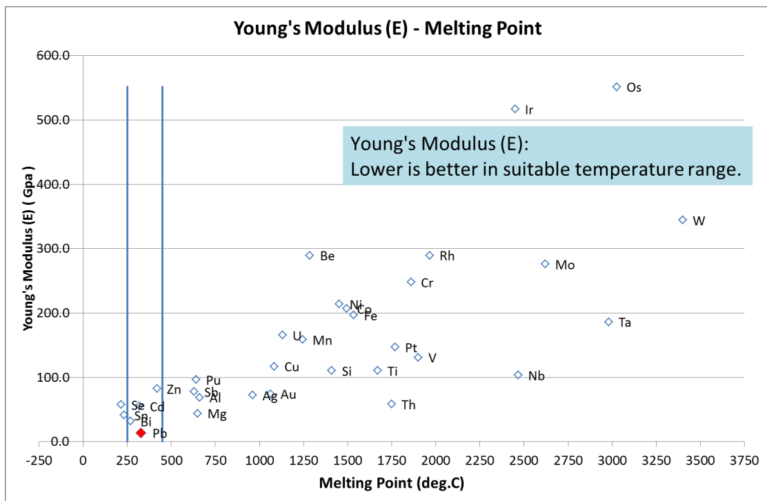
Graph 5: Young's Modules (E) (an indication of ductility) – Melting Point. (Wide temperature range)
