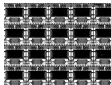
Scanning acoustic microscopy shows delamination of large power transistor die attach after 1000 th. cycles -50°C / +150°C
