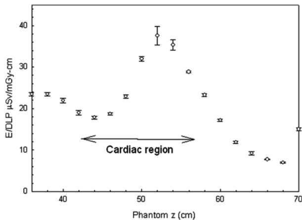
FIGURE 4. Values of E/DLP for 4-cm scan lengths in the chest region as a function of the long patient axis location ( z ) shown in Figure 1, obtained using ICRP 103 weighting factors.
