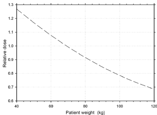
FIGURE 2. Changes in dose to organs in the chest as a function of patient weight at a constant incident radiation intensity (CTDI vol and DLP). Doses have been normalized to unity for a 70-kg adult.
