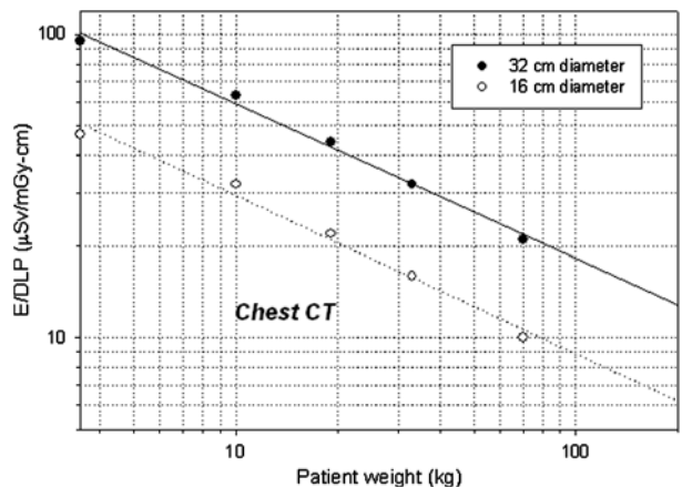
FIGURE 3. E/DLP conversion factors for chest CT examinations as a function of patient weight, obtained using ICRP 103 weighting factors. Closed circles are for DLP in 32-cm diameter acrylic phantoms, and open circles are for DLP in 16-cm diameter acrylic phantoms.
